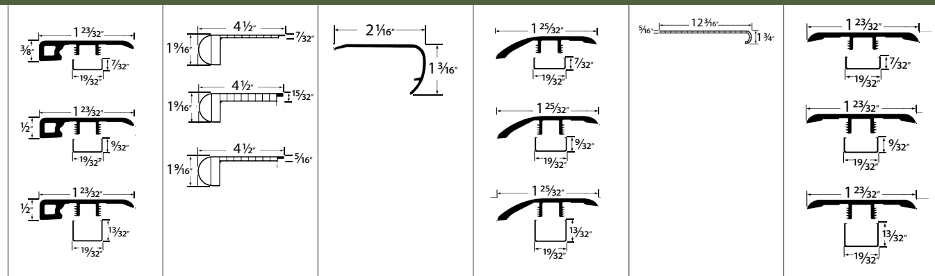
Overlap Stairnose Covers stair edge overlap
